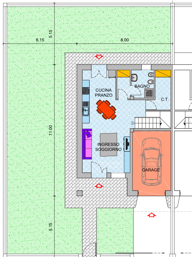
PIANO TERRA
